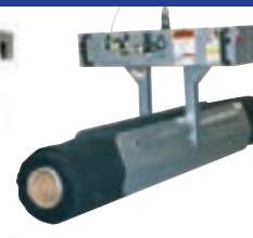
VODC Pneumatic OD Clamp Lifter 330 lbs. (150 kg) Any Roll Diameters & Widths
